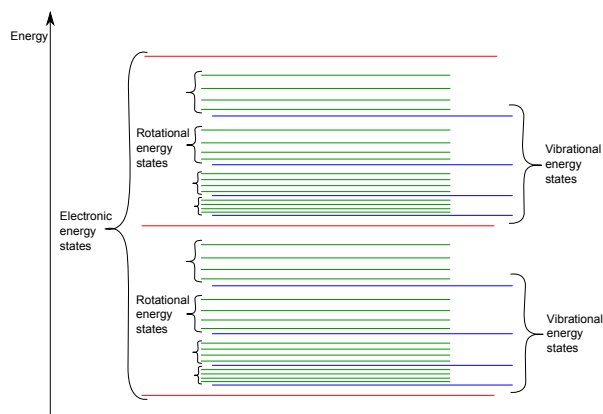
Fig. 5 Simplified illustration of the electronic, vibrational, and rotational energy states. Each line illustrates a discrete energy level that the molecule can exist in.
