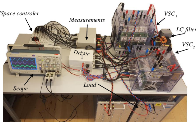
Fig. 12. Experimental setup.
