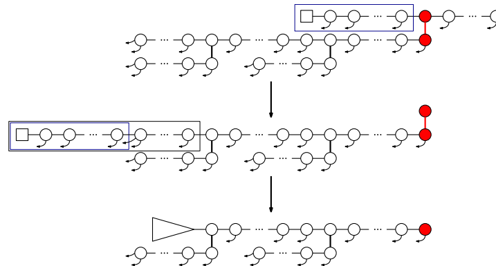
Figure 55: Transforming R_{2,1} into an instance of R_1 .
