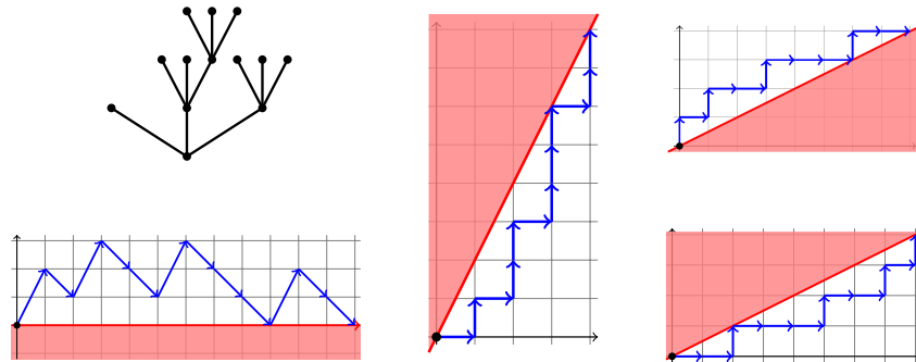
Figure 24: Examples of combinatorial structures which are in bijection: ternary trees, excursions of directed lattice paths with jumps +2 and -1 , Dyck paths of North-East steps below the line y = 2x , Dyck paths above the line y = \frac{1}{2}x , and Dyck paths below the line y = \frac{1}{2}x .
