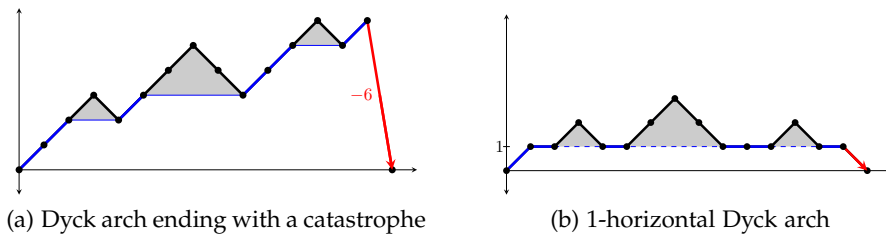
Figure 35: The bijection of Theorem 6.2.1 transforming Dyck arches ending with catastrophes into 1-horizontal Dyck arches, and vice versa.
