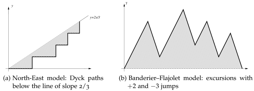
Figure 31: Dyck paths below the line of slope 2/3 and Duchon's club histories (i.e., excursions with jumps +2, -3 ) are in bijection. Duchon conjectured that the average area (in gray) after n jumps is asymptotically equal to Kn^{3/2} ; our approach shows that K = \sqrt{15\pi}/2 .
