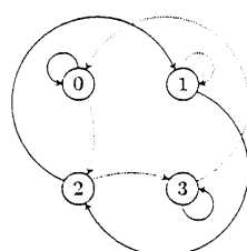
The graph B_1^{(4)}[\delta_3] \cup B_1^{(4)}[\delta_4]
