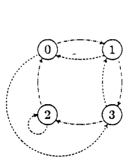
The graph B_1^{(4)}[\delta_1] \cup B_1^{(4)}[\delta_2]
