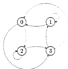
The graph B_1^{(4)}[\delta_2] \cup B_1^{(4)}[\delta_3]
