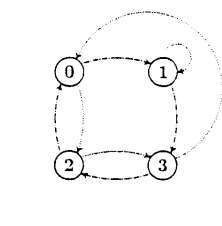
The graph B_1^{(4)}[\delta_1] \cup B_1^{(4)}[\delta_3]
