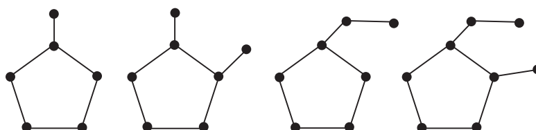
Figure 1: Some light graphs in \mathcal{G}(3, 5)
