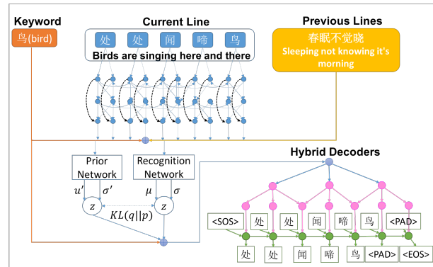
Figure 2: The training procedure of the proposed Conditional Variational Autoencoders with Hybrid Decoders. The black dashed lines represent the residual connection between layers.
