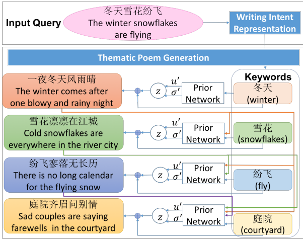
Figure 1: The framework of the proposed Chinese poetry generation approach. \oplus denotes the concatenation of input vectors.
