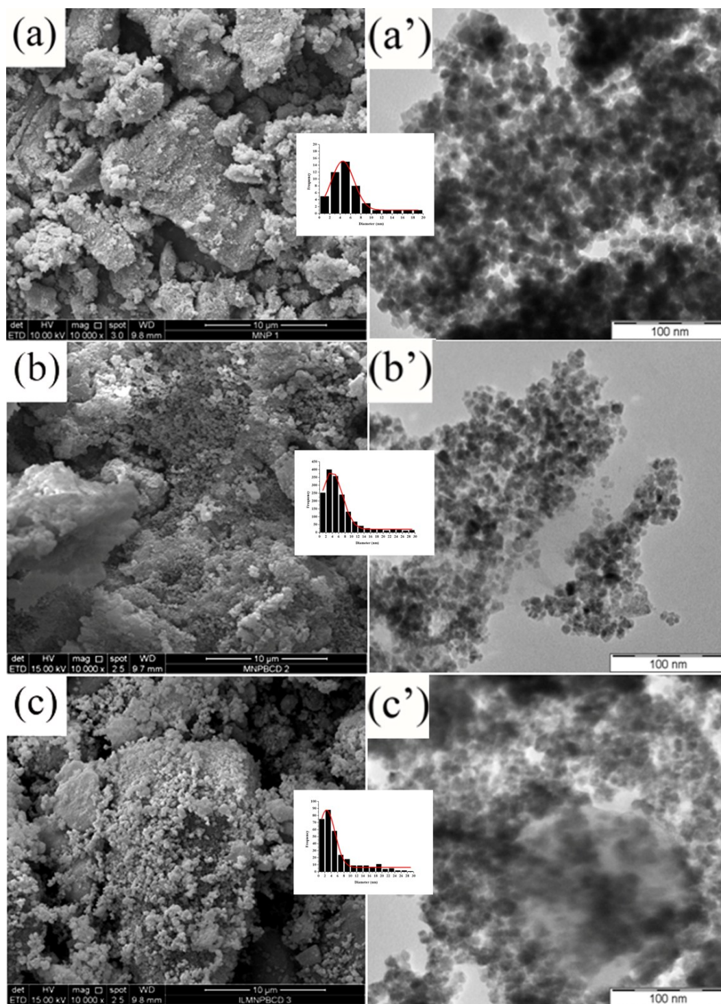
Fig. S1. IMAGE J analysis and SEM images of (a) MNP, (b) MNP- \beta CD-TDI, and (c) IL-MNP- \beta CD-TDI, as well as TEM images of (a') MNP, (b') MNP- \beta CD-TDI, and (c') IL-MNP- \beta CD-TDI.
