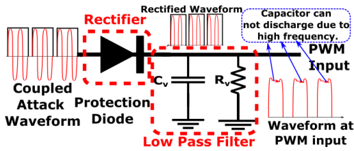
Figure 5: The protection diode rectifies the attack waveform. The victim capacitance ( C_v ) is charged up to the peak but not able to discharge which results in the appearance the attack waveform envelope at the PWM input.
