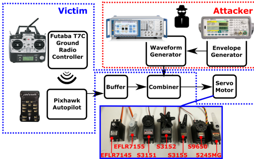
Figure 3: The reported attack waveforms are tested in a wired experimental setup on different servo models.
